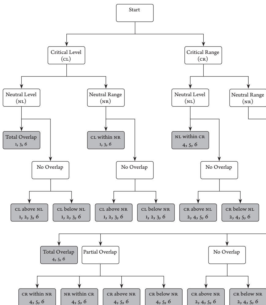
FIGURE 1 Taxonomy
